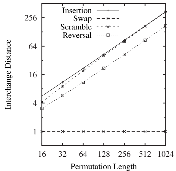
Figure 5: Average Interchange Distance between parent and child permutations produced by 1 random mutation.
